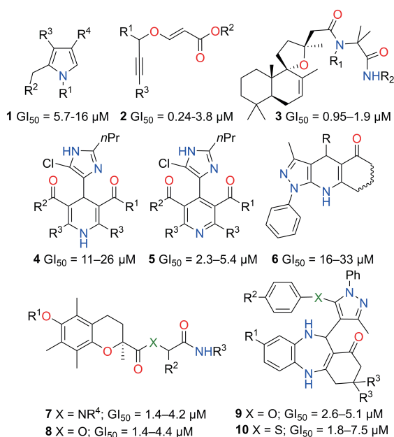
Figure 1. General structure of scaffolds obtained by MCRs, with indication of the anti-proliferative activity ( \text{GI}_{50} ) of the resulting leads.
