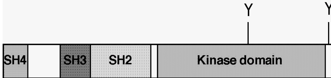
Figure 3. The domain structure of the Src protein tyrosine kinase family.
