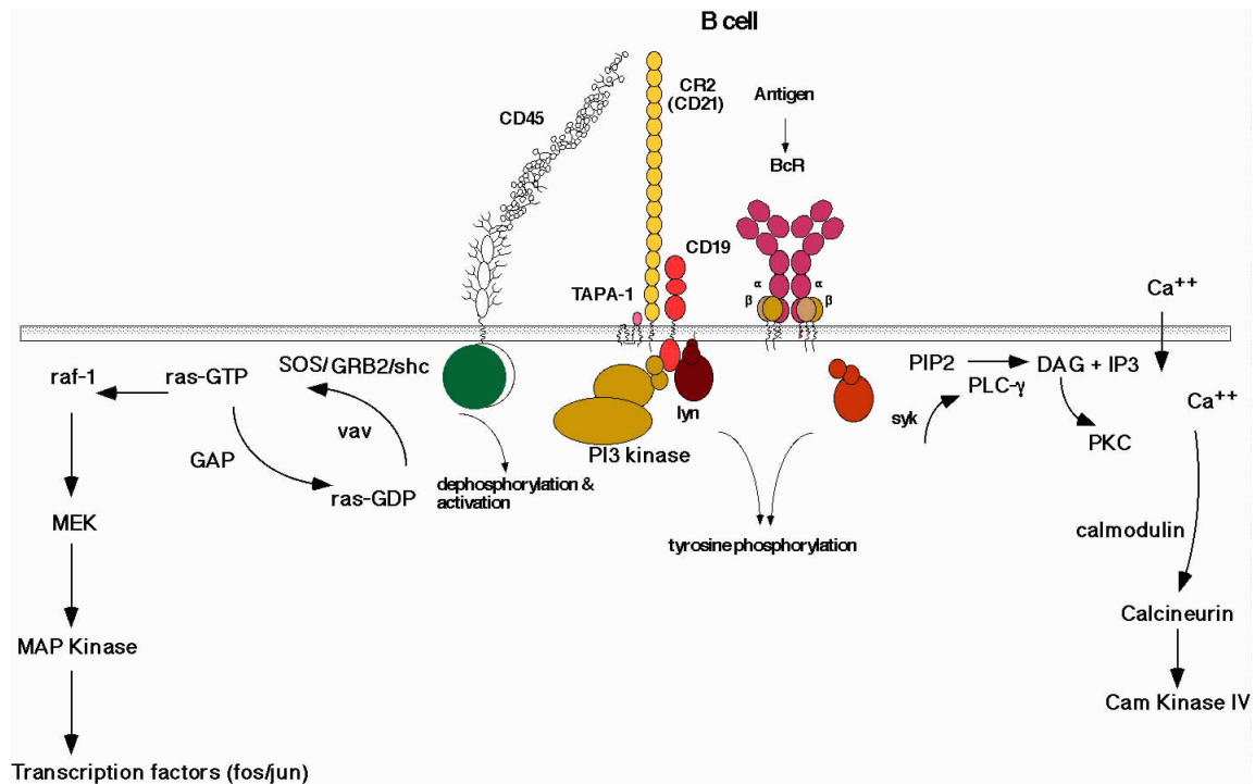
Figure 2. Regulation of antigen receptor-mediated signal transduction in B cells.
