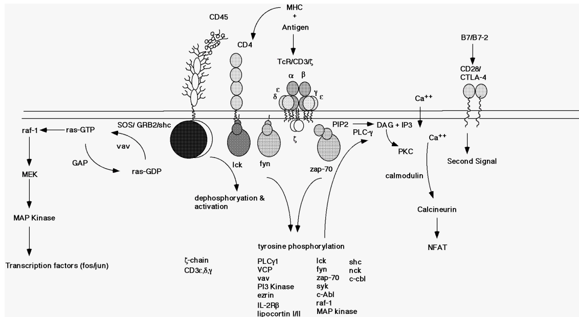
Figure 1. Regulation of antigen receptor-mediated signal transduction in T cells.
