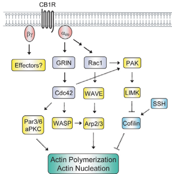
Figure 4. G i/o signaling to the actin cytoskeleton during the induction of neurite outgrowth. Signaling from the G i/o -coupled CB1R to its effectors GRIN, Cdc42 and Rac1 and their potential downstream targets is shown in the schematic. The intermediate molecules between CB1R and Rac1 have been omitted for clarity. It is likely that Gβγ also signals to yet to be identified downstream effectors to reorganize the actin cytoskeleton. Known interactions are depicted by solid arrows, putative interactions by dashed arrows. See text for further details. PAK, p21-activated kinase; SSH, Slingshot; WASP, Wiskott-Aldrich-syndrome protein.
