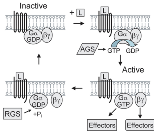
Figure 1. Heterotrimeric G-protein mechanism. The activation of the G-protein coupled receptor by a ligand (L) causes the exchange of GDP for GTP on the \alpha subunit. This switches G\alpha to the active conformation and results in the release of G\alpha and G\beta\gamma from the receptor to signal to downstream effectors. The switch is turned off by the intrinsic GTP hydrolysis (GTPase) activity of G\alpha , which leads to its reassociation with G\beta\gamma and the receptor. The regulators of G-protein signaling (RGS) play key roles in inactivating G-protein signaling. The activators of G-protein signaling (AGS) activate G-proteins by several mechanisms.
