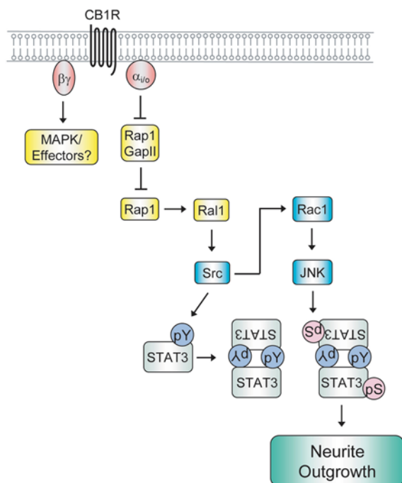
Figure 3. G i/o signaling to the nucleus during the induction of neurite outgrowth. Signal flow emanating from stimulation of the G i/o -coupled cannabinoid receptor 1 (CB1R) to the activation of the transcription factor STAT3 is depicted in the schematic. It is likely that Gβγ also signals to downstream effectors to change patterns of gene expression, possibly through p42/44 mitogen activated protein kinase (MAPK). See text for further details. pY, phospho-tyrosine; pS, phospho-serine.
