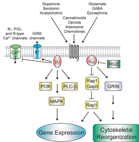
Figure 2. Effector pathways activated by G i/o signaling. Signals from a wide array of hormones, neurotransmitters, and chemokines are transduced into intracellular responses by G i/o -coupled receptors. Depicted are pathways that are stimulated by Gα and Gβγ and lead to changes in gene expression and cytoskeletal reorganization. See text for further details. GIRK, G-protein-coupled inward rectifying potassium channels.
