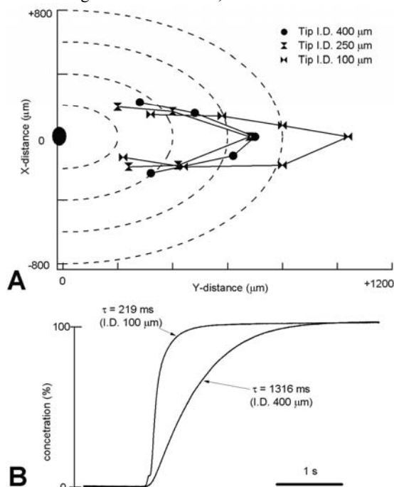
Figure 6. Effects of delivery tip I.D. (A) C90 with three pipettes of differing I.D. Test condition: reservoir height = 40 cm, Angle = 45^\circ , Flow rate = 18 s/drops; arrangement as for Figure 4B. (B) Examples of delivery kinetics with 100 and 400 \mu\text{m} I.D. pipettes.
