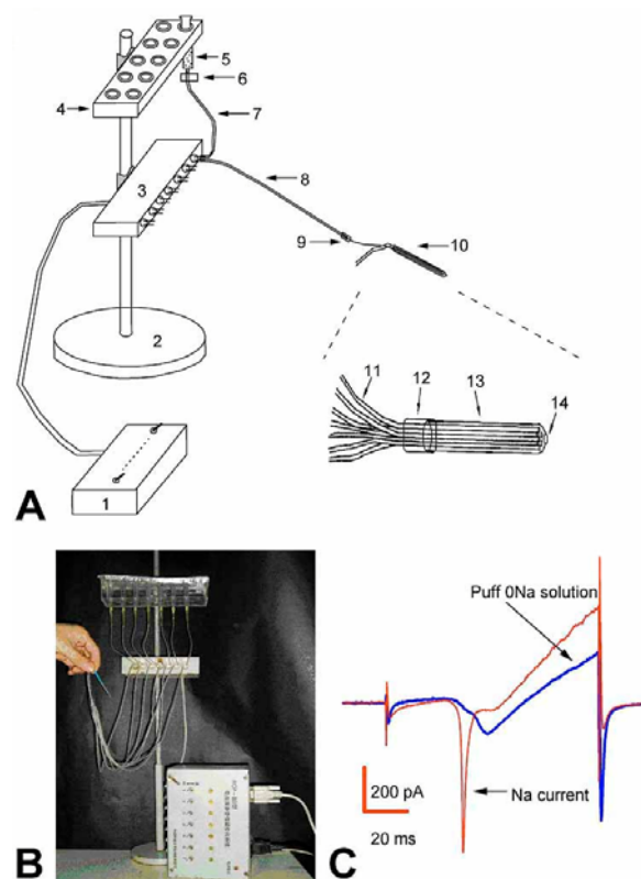
Figure 1. The RCP-II drug puffer system. A: Schematic diagram of the system. (1-controller, 2-base, 3-valves, 4-syringe holder, 5- syringes, 6-manual three-way stopcock, 7,8-emulsion tubes (I.D. >1 mm), 9-tubing adapter, 10,13-glass puffing pipette, 11-polyethylene tubes (I.D. = 0.28 \mu m), 12-adhesive, 14-pipette tip (I.D. = 100-200 \mu m). B: Photograph of the RCP-II system. C: Biological application: Blockade of sodium current during standard whole-cell voltage clamp recording from cultured chromaffin cells. In the presence of sodium-containing solution, a prominent sodium current was detected as the voltage ramp was applied (red trace). When sodium-free solution was applied through the puffer pipette of the RCP-II system, the same ramp failed to generate a current (blue trace).
