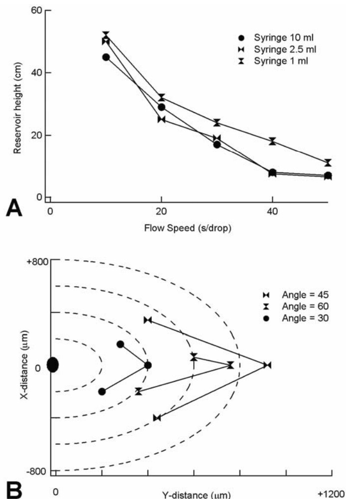
Figure 4. Effect of reservoir height and pipette angle. (A) Effect of reservoir height (cm) on flow rate (seconds per drop) for 10 ml, 2.5 ml and 1 ml syringes. (B) Effect of pipette angle on territory under control. Test conditions: reservoir height = 40 cm, flow rate = 18 s/drop, tip I.D. = 100 \mu m. The recording pipette was placed at various distances up to 1200 \mu m from the puffing tip, which was fixed at 0,0, indicated by the small grey circle on the x-axis.
