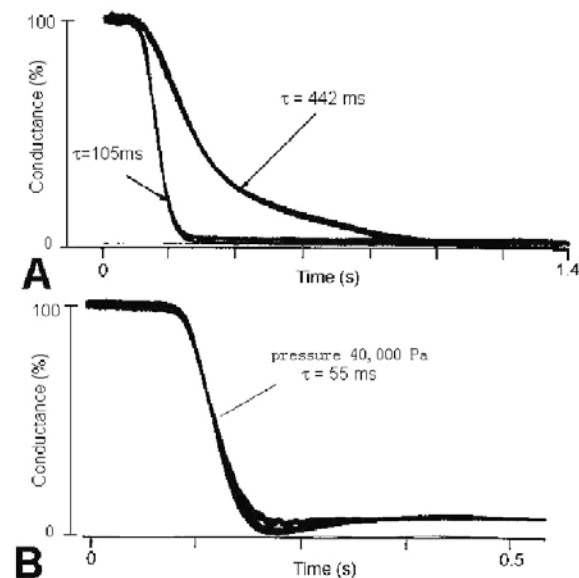
Figure 3. Effect of connecting tube diameter on puffing kinetics. (A) Puffing kinetics of two types of connection tubing ( \tau = 105 ms using 2 mm emulsion tubing, \tau = 442 ms using 0.28 mm polyethylene tubing) at ambient atmospheric pressure. The “%-conductance” is the inverse value of “%-concentration” of the applied drug (distilled water in this case). (B) After applying an external pressure of 4 \times 10^4 Pa, the kinetics became the same for both types of tubing ( \tau = 55 ms).
