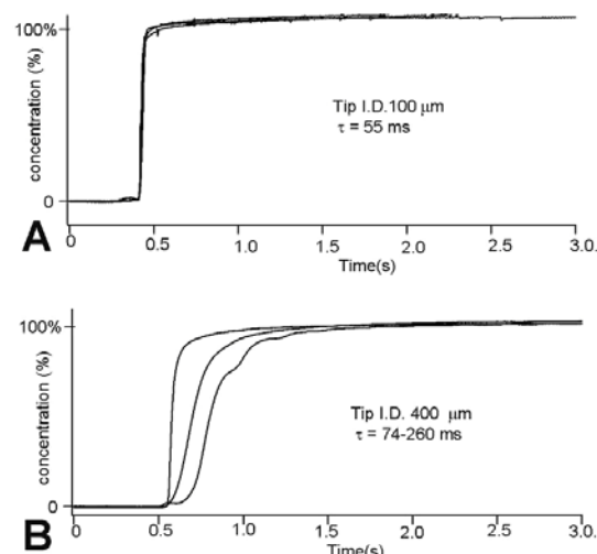
Figure 2. Consistency of drug-delivery kinetics among different tubes. Superimposed traces from a sensing electrode to puffs from each of the seven tubes in one puffing pipette. Note that the puffing tip with 100 \mu\text{m} tip diameter evoked fast and consistent responses (A), while in a 400 \mu\text{m} tip, different tubes evoked significantly different response kinetics (B).
