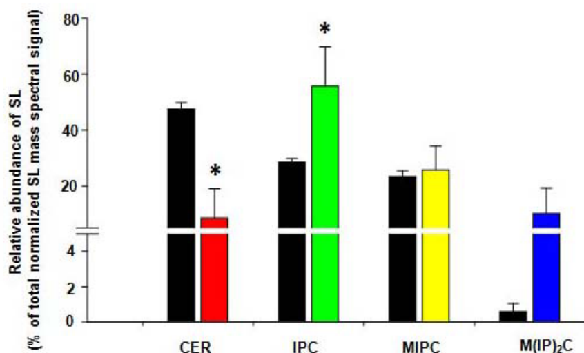
Figure 3. Effect of CUR on SLs composition. Figure shows the relative abundance of SL groups as mole percentage of the normalized total SL mass spectral signal. The total for each SL class was calculated by adding the mole percentage of the molecular lipid species of that class. The entire data set is shown in the table (Table 1). Values are means \pm SD ( n = 3 ). Statistically significant ( p -value < 0.05 ) differences are marked by an asterisk (*). The black bars represent the untreated cells and the colored bars are the CUR treated cells.
