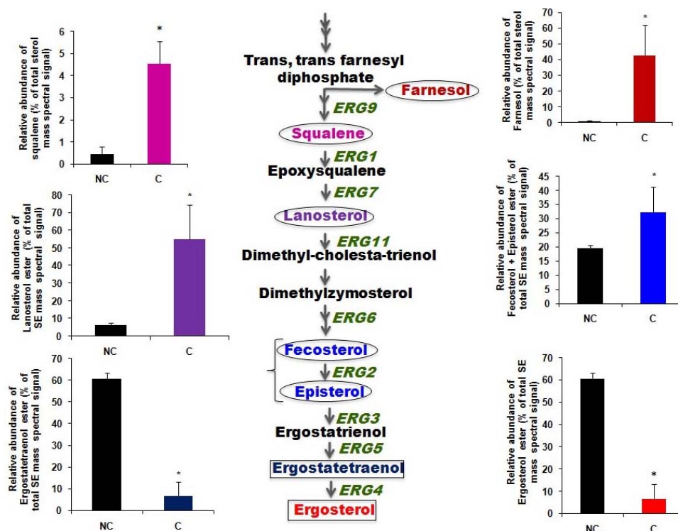
Figure 3. Effect of CUR on SLs composition. Figure shows the relative abundance of SL groups as mole percentage of the normalized total SL mass spectral signal. The total for each SL class was calculated by adding the mole percentage of the molecular lipid species of that class. The entire data set is shown in the table (Table 1). Values are means \pm SD ( n = 3 ). Statistically significant ( p -value < 0.05 ) differences are marked by an asterisk (*). The black bars represent the untreated cells and the colored bars are the CUR treated cells.
